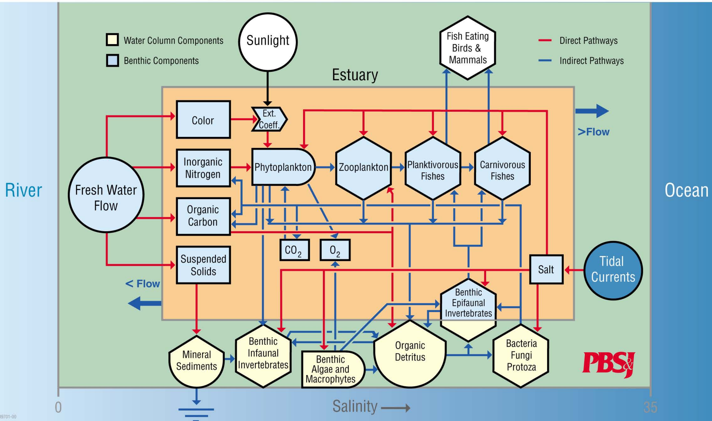
Figure 3.4 Conceptual Model of the Peace River Estuarine System
