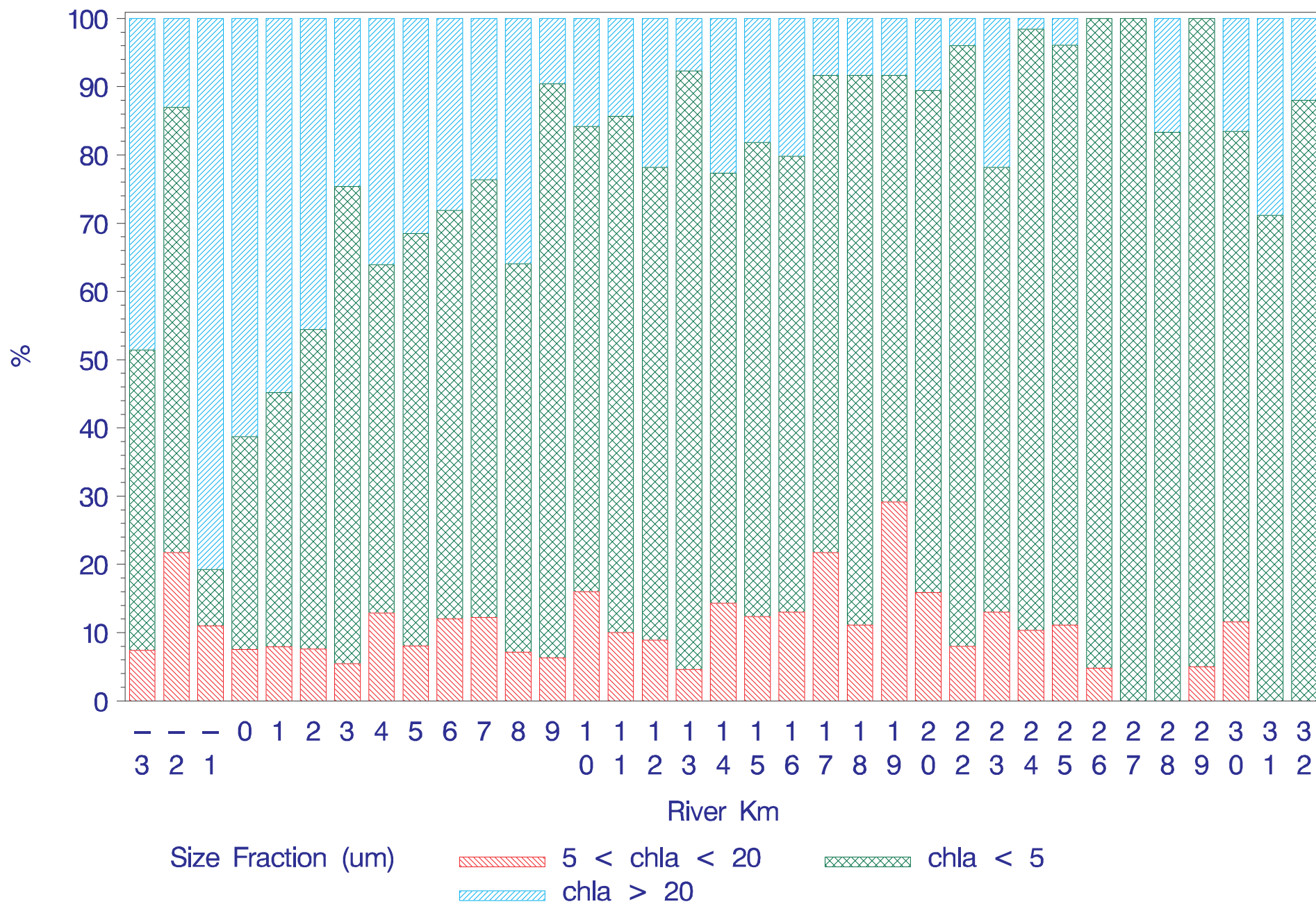
Chlorophyll Size Fraction (%) vs. River Km 1996–1998 Surface
