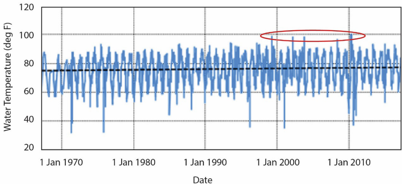
Figure 18. Water temperature in Sarasota Bay. Source: adapted from USF Water Institute 2017.
