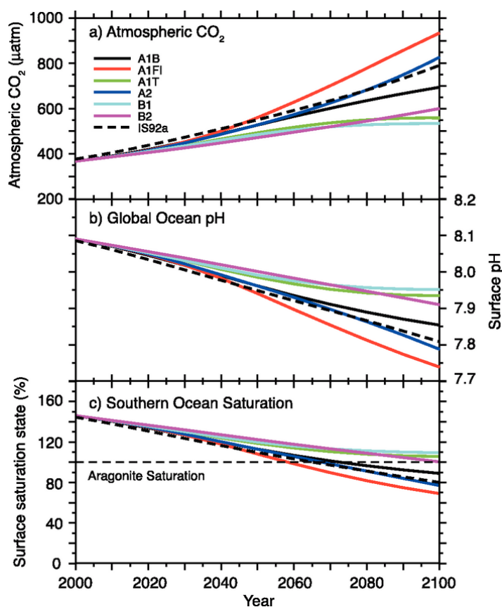
Figure 19 (top) Projected atmospheric CO 2 for the six IPCC Special Reports on Emission Scenarios (SRES); (middle) projected global average surface pH; (bottom) projected average saturation state of aragonite in the Southern Ocean. Source: modified from Orr et al. (2005) as cited in IPCC 2007.
