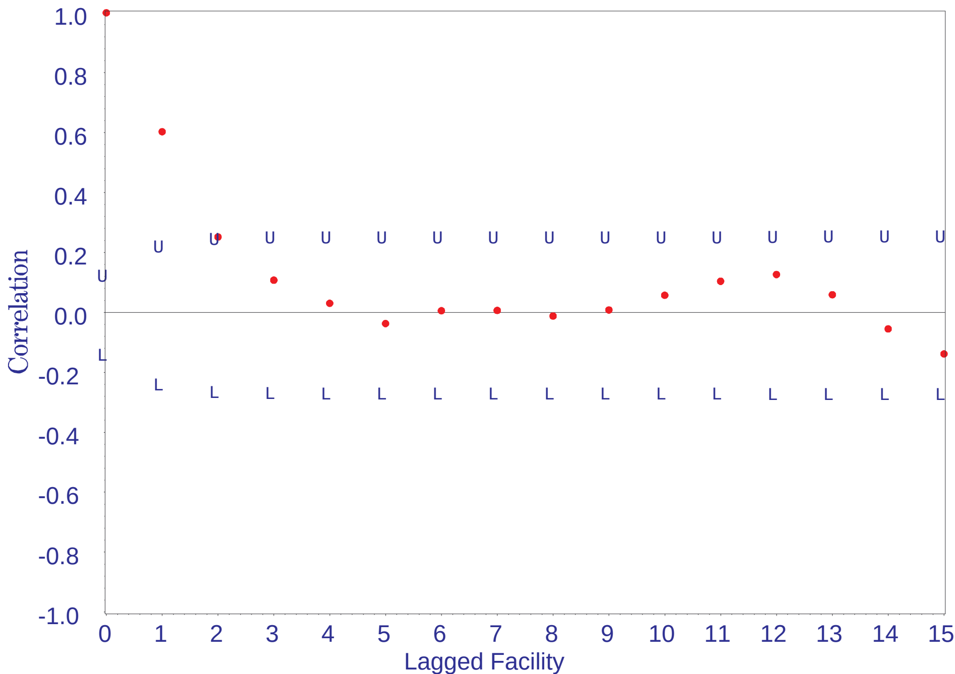
River Flow at Treatment Facility (cfs) 1980-1998 Correlogram with Upper and Lower 95% Confidence Limits
