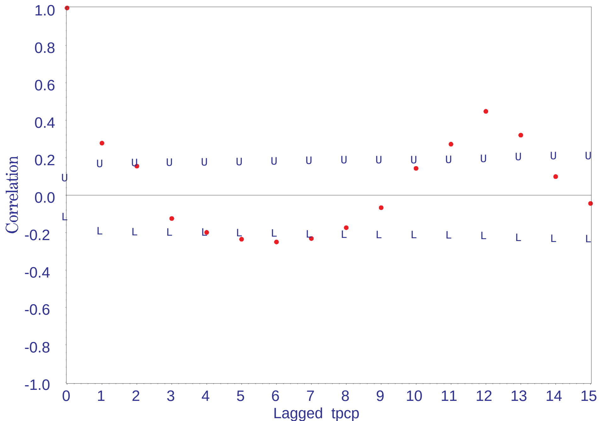
Monthly Rainfall at the Bartow Gauge 1966-1998 Correlogram with Upper and Lower 95% Confidence Limits
