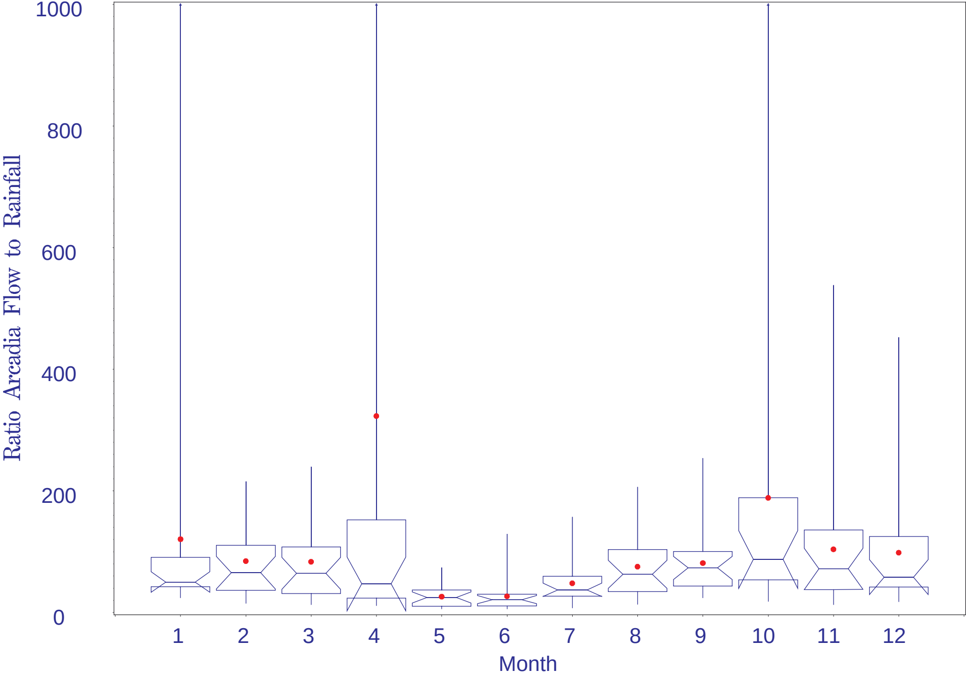
Ratio Arcadia Flow to Rainfall (Arcadia + Wachula + Bartow) 1976-1998 Monthly Boxplots
