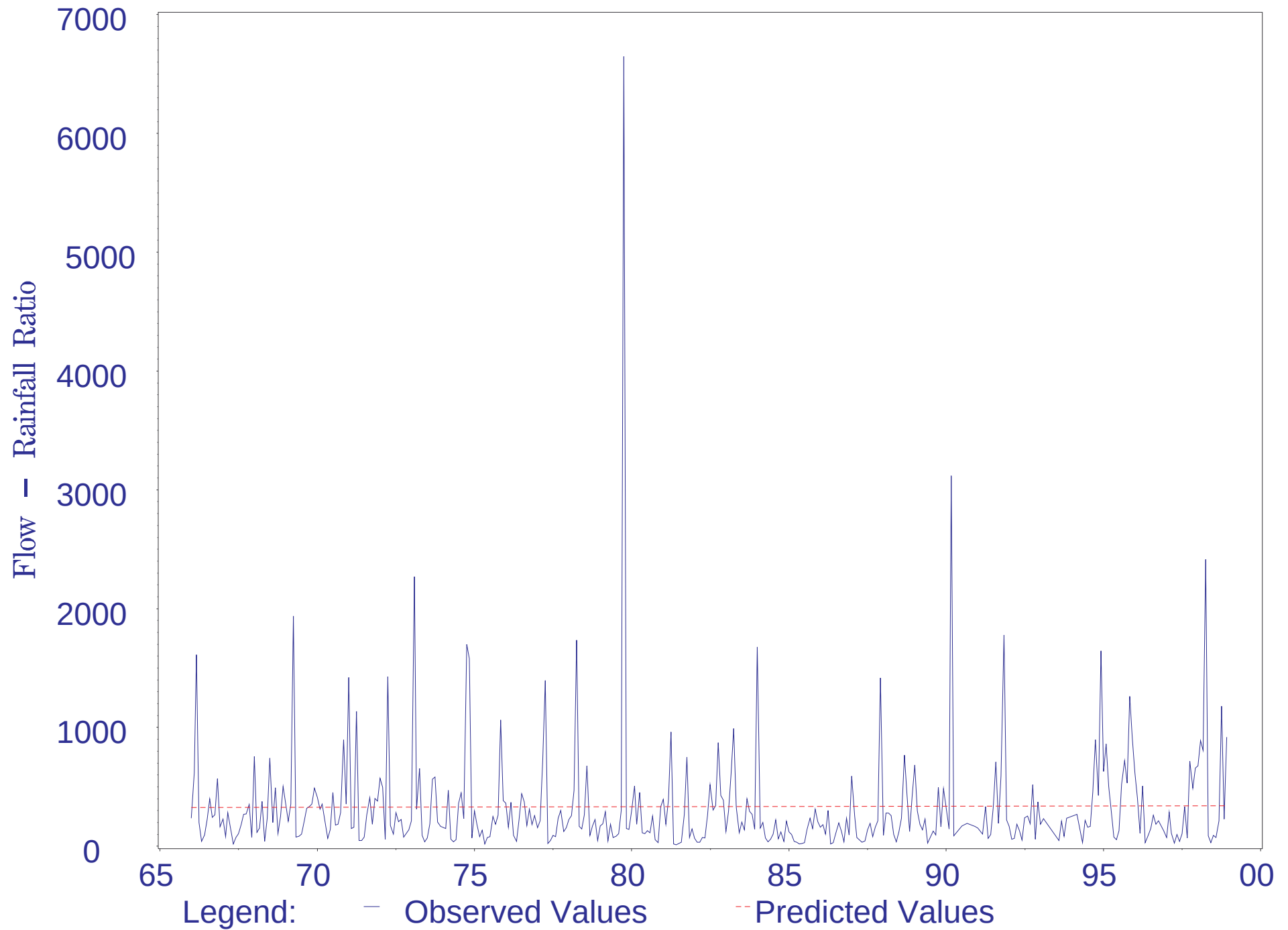
Ratio Arcadia Flow to Arcadia Rainfall (1966-1998)
