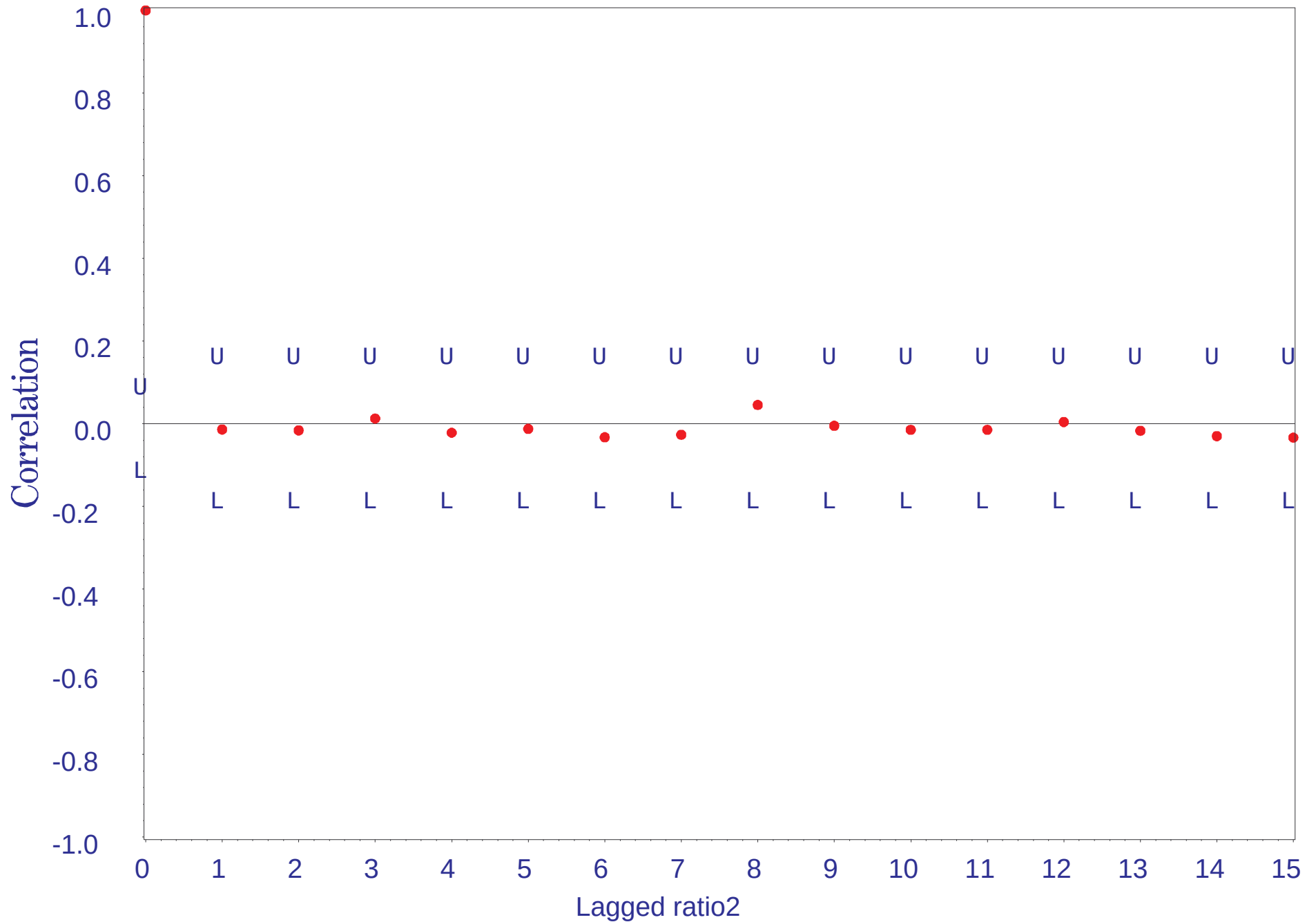
Ratio Arcadia Flow to Rainfall (Sum Arcadia + Wachula + Bartow) 1966-1998 Correlogram with Upper and Lower 95% Confidence Limits
