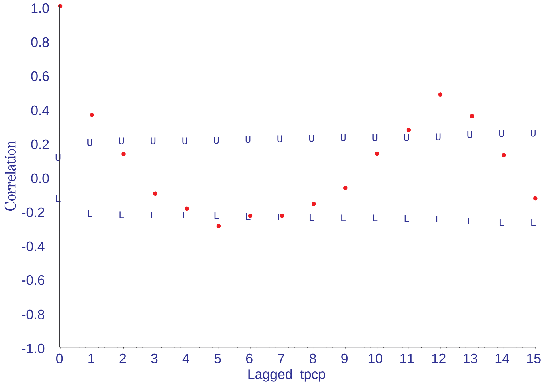
Monthly Rainfall at the Wauchula Gauge 1976-1998 Correlogram with Upper and Lower 95% Confidence Limits
