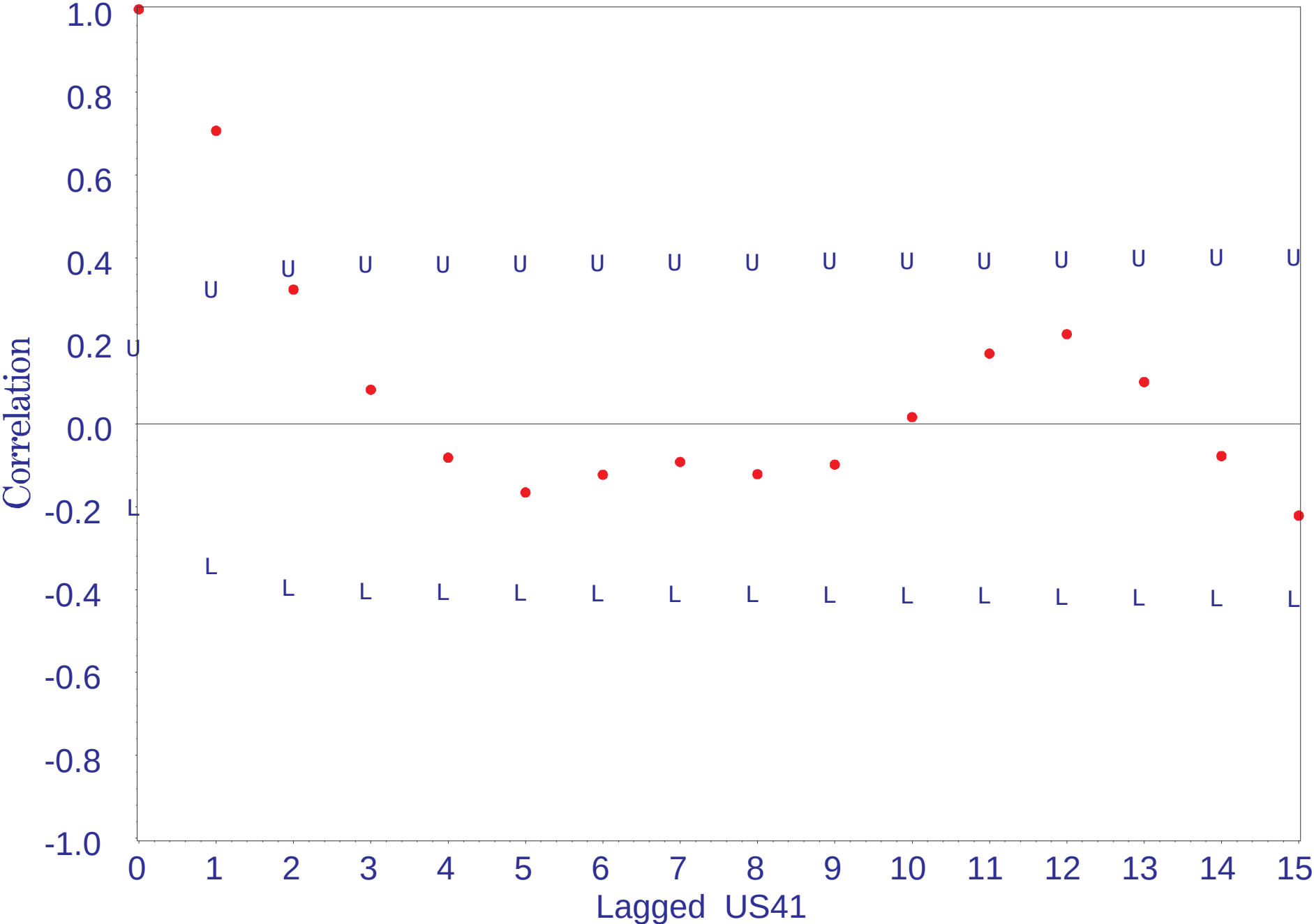
River Flow at US 41 Bridge 1990-1998 Correlogram with Upper and Lower 95% Confidence Limits
