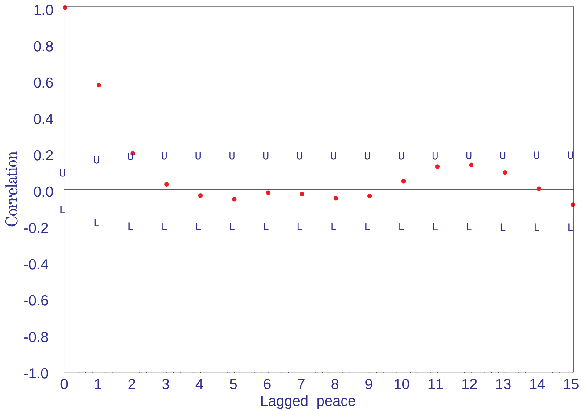
Peace River Flow (cfs) 1966-1998 Correlogram with Upper and Lower 95% Confidence Limits C-33
