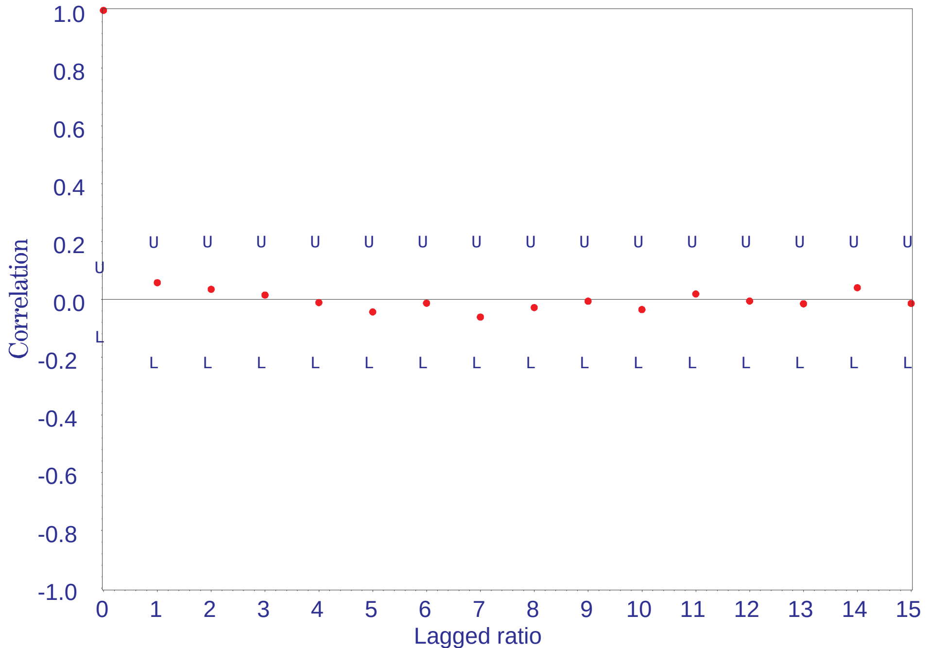
Ratio Arcadia Flow to Arcadia Rainfall (1976-1998) Correlogram with Upper and Lower 95% Confidence Limits
