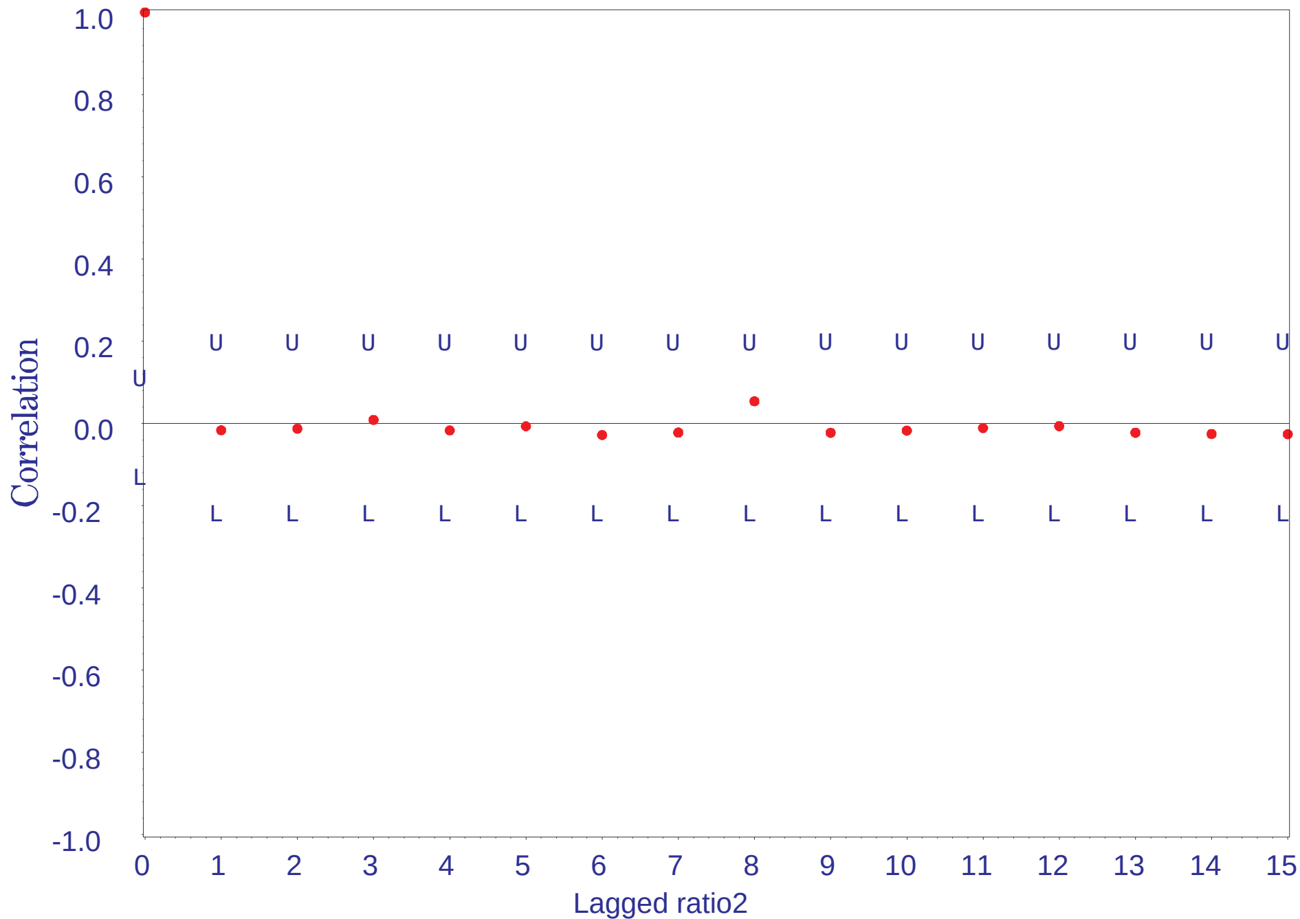
Ratio Arcadia Flow to Rainfall (Arcadia + Wachula + Bartow) 1976-1998 Correlogram with Upper and Lower 95% Confidence Limits
