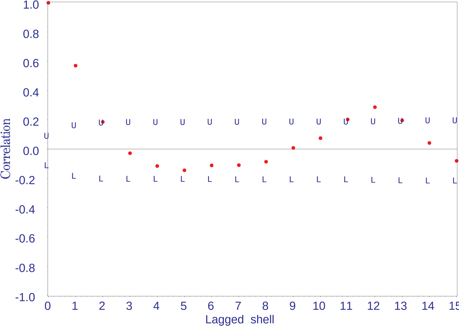
Shell Creek Flow (cfs) 1966-1998 Correlogram with Upper and Lower 95% Confidence Limits C-45
