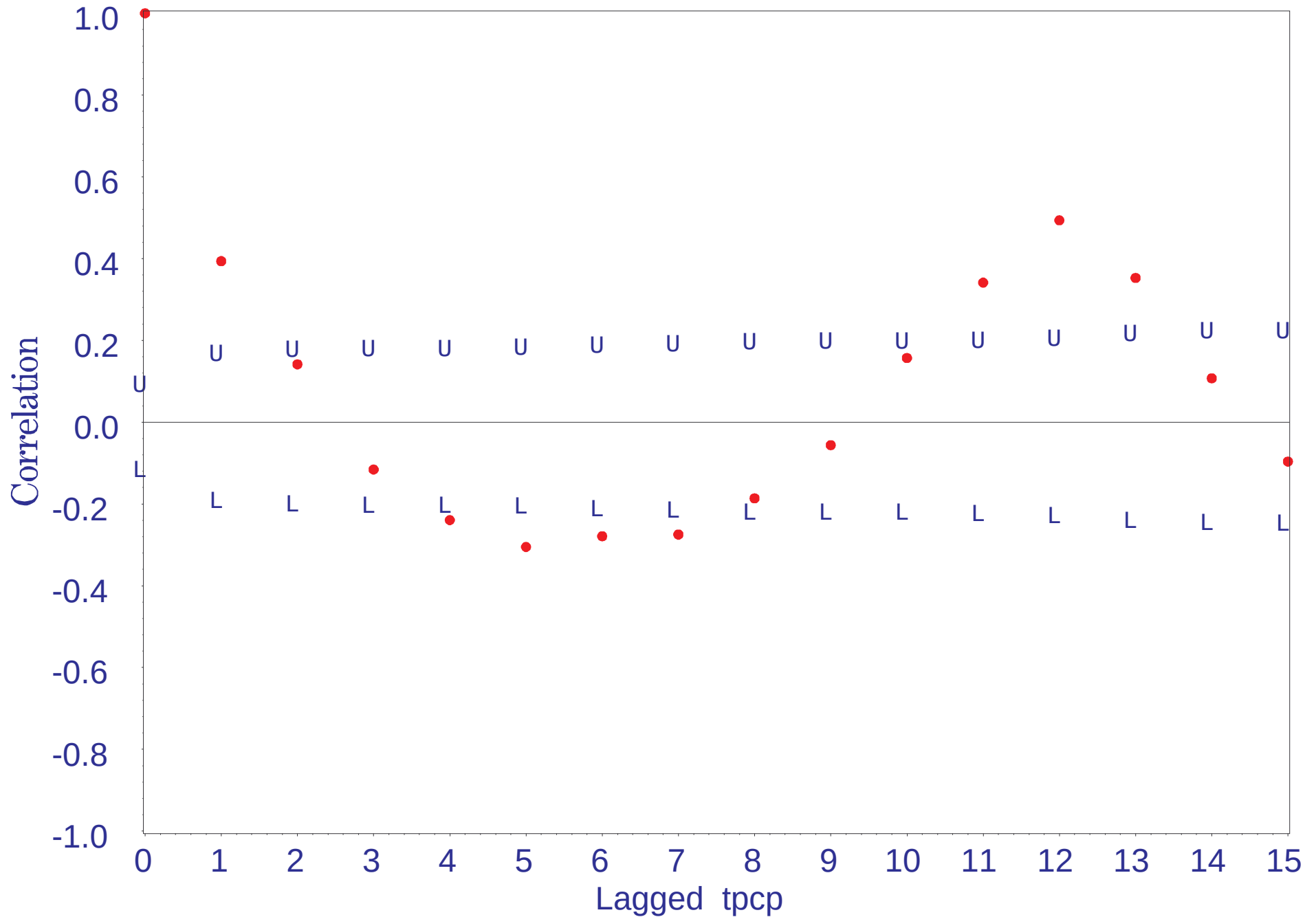
Monthly Rainfall at the Wauchula Gauge 1966-1998 Correlogram with Upper and Lower 95% Confidence Limits
