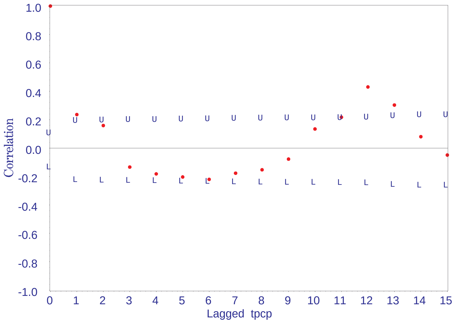
Monthly Rainfall at the Bartow Gauge 1976-1998 Correlogram with Upper and Lower 95% Confidence Limits
