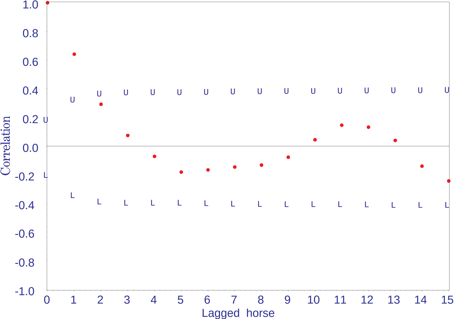
Horse Creek Flow (cfs) 1990-1998 Correlogram with Upper and Lower 95% Confidence Limits
