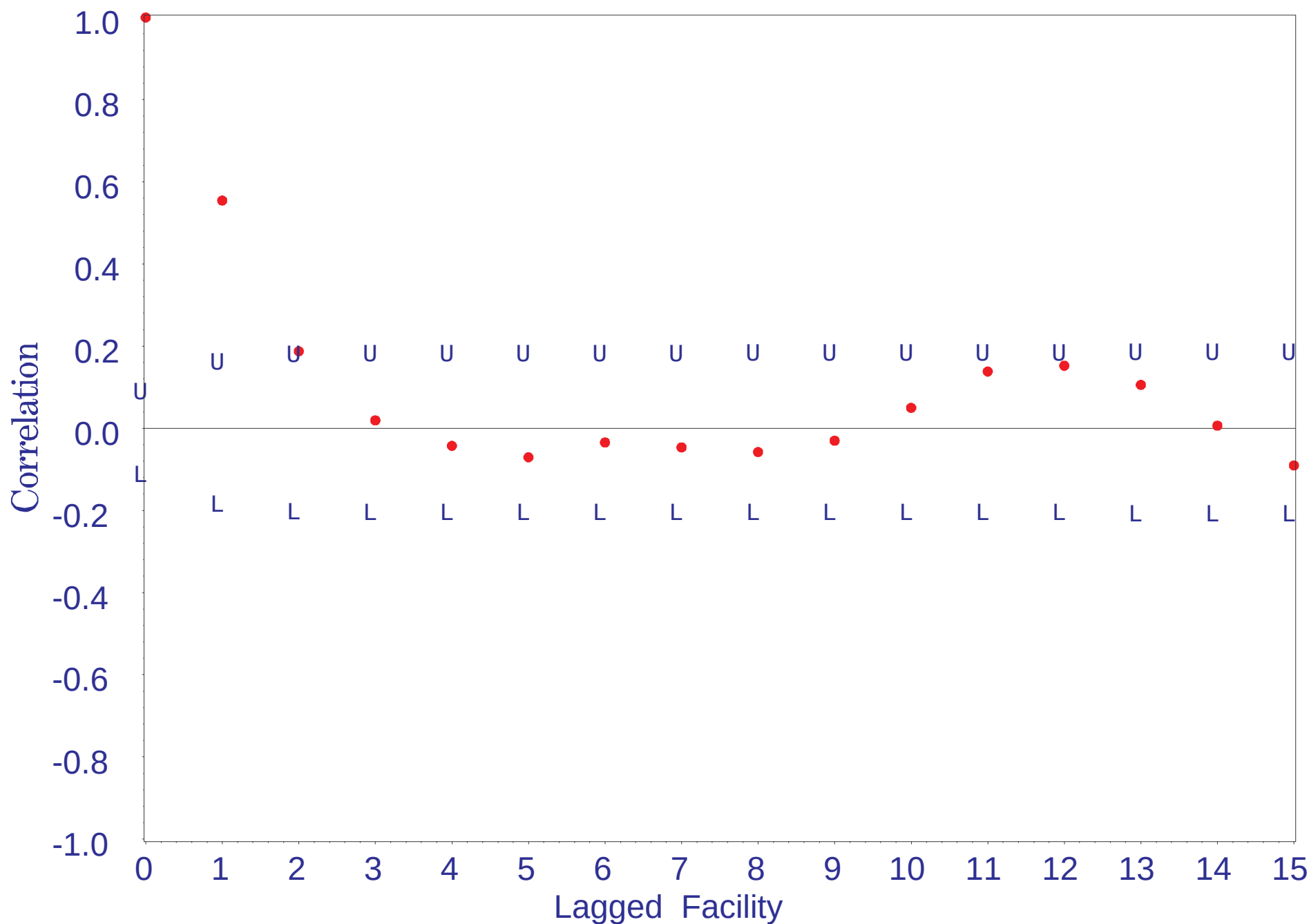
River Flow at Treatment Facility (cfs) 1966-1998 Correlogram with Upper and Lower 95% Confidence Limits
