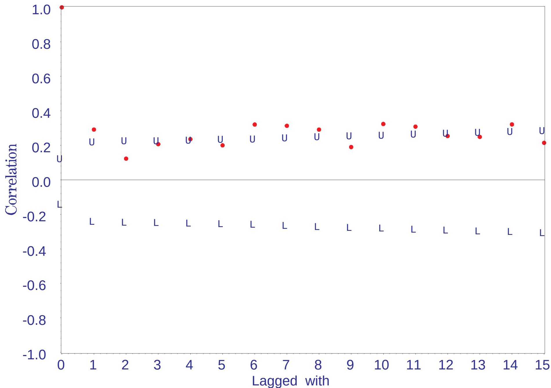
Treatment Facility Withdrawals 1980-1998 Correlogram with Upper and Lower 95% Confidence Limits
