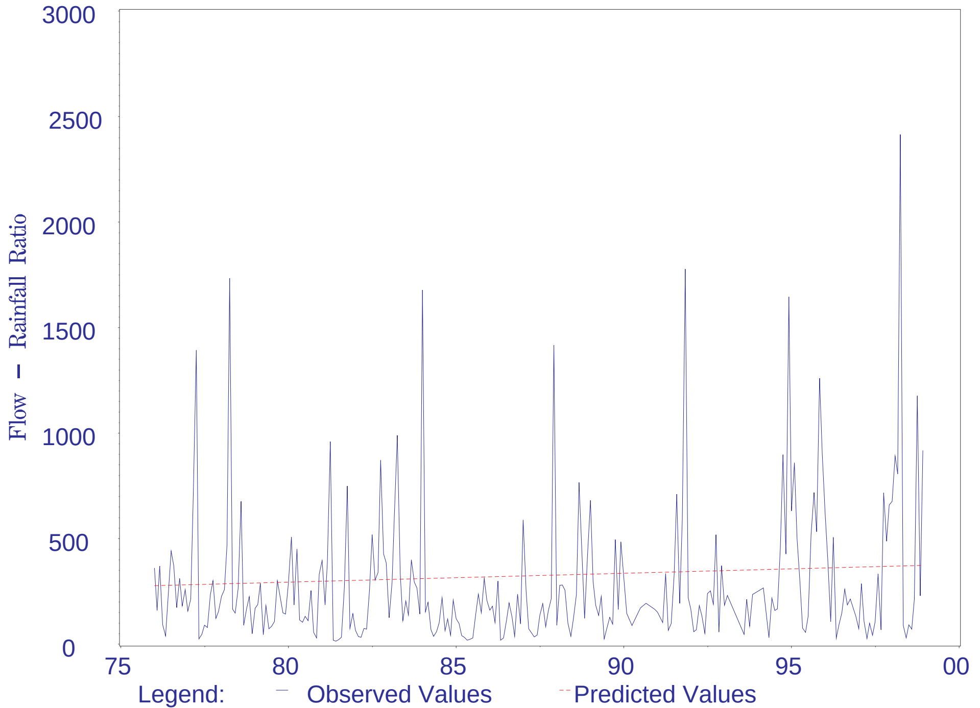
Ratio Flow at Arcadia to Rainfall at Arcadia (1976-1998)
