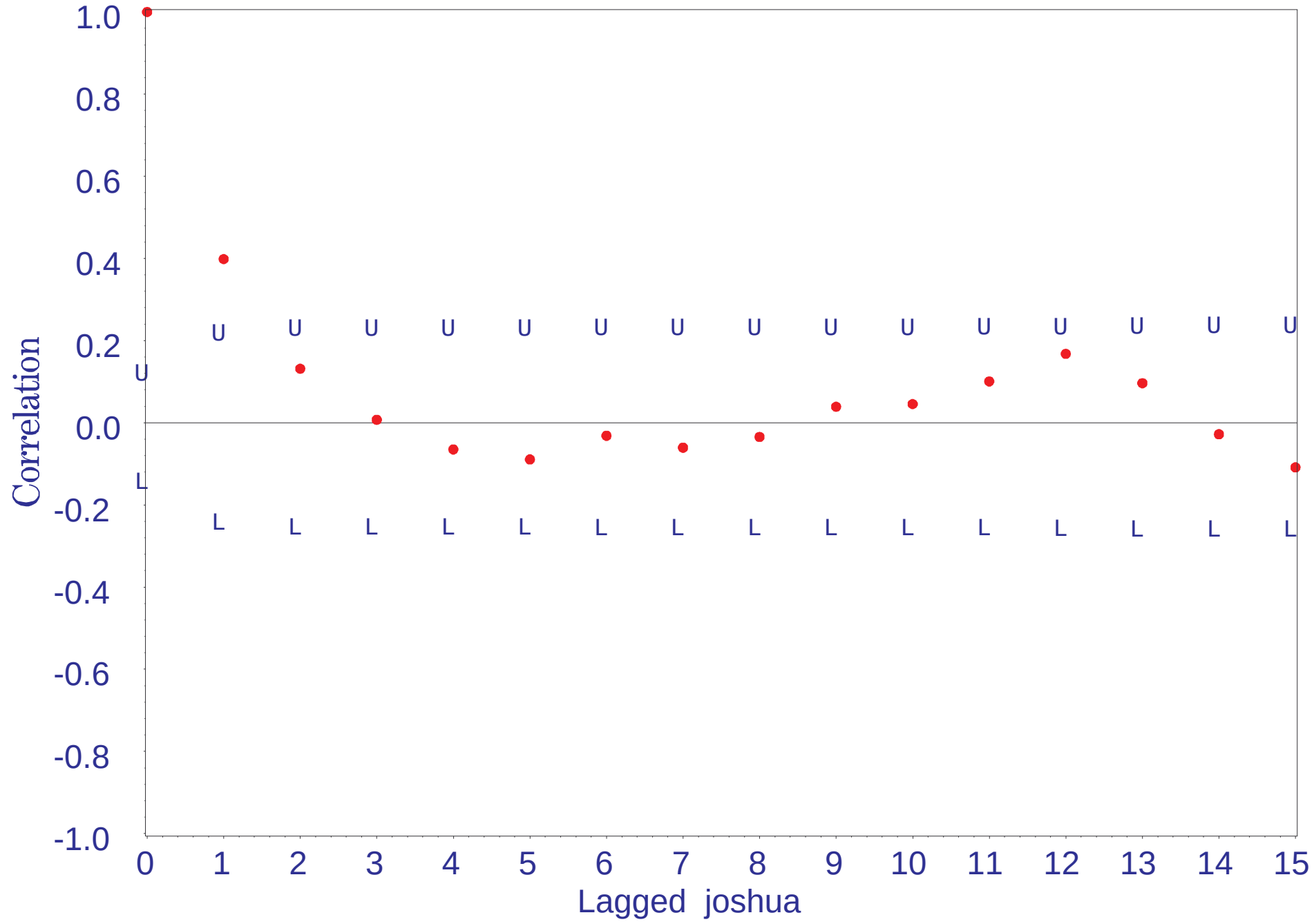
Joshua Creek Flow (cfs) 1980-1998 Correlogram with Upper and Lower 95% Confidence Limits C-57
