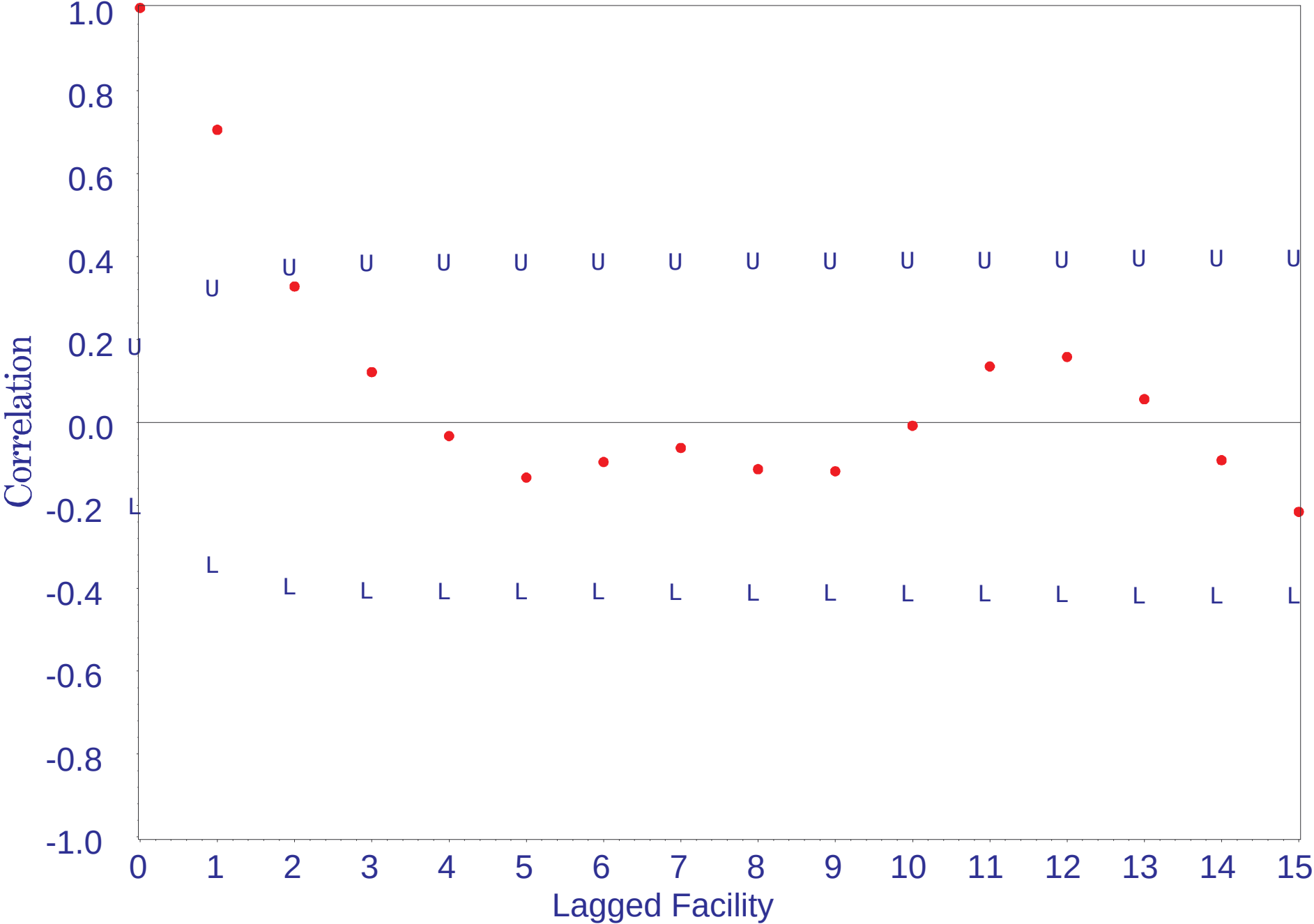
River Flow at Treatment Facility (cfs) 1990-1998 Correlogram with Upper and Lower 95% Confidence Limits
