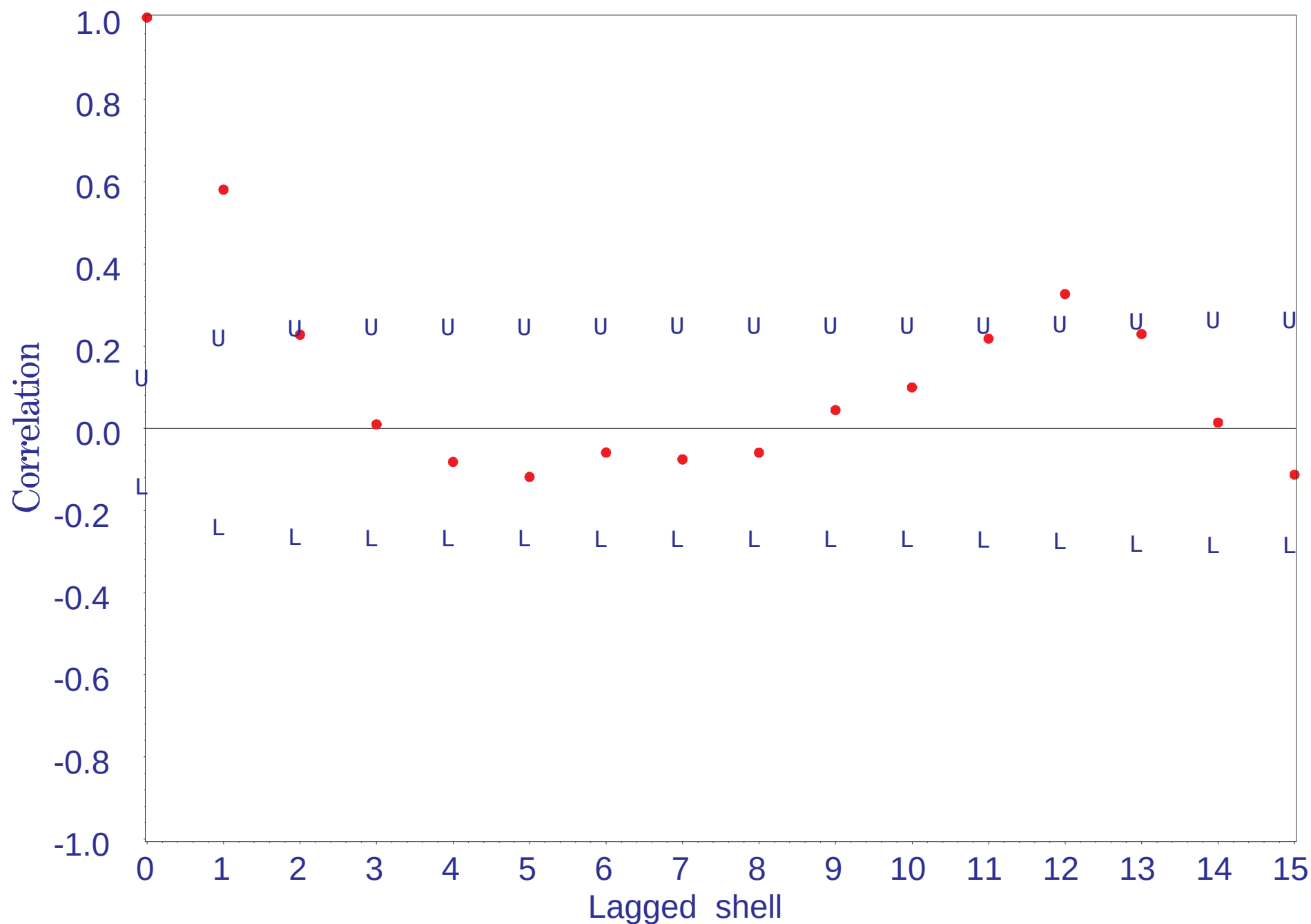
Shell Creek Flow (cfs) 1980-1998 Correlogram with Upper and Lower 95% Confidence Limits
