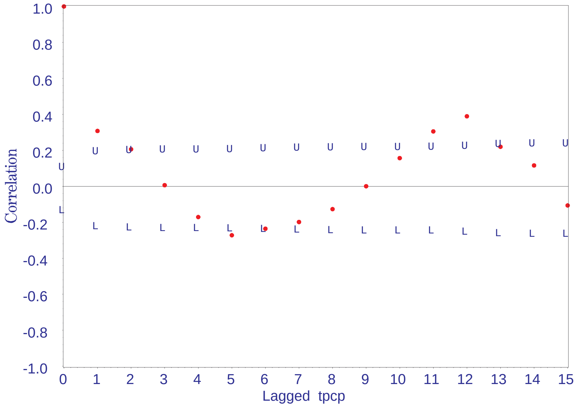
Monthly Rainfall at the Arcadia Gauge 1976-1998 Correlogram with Upper and Lower 95% Confidence Limits
