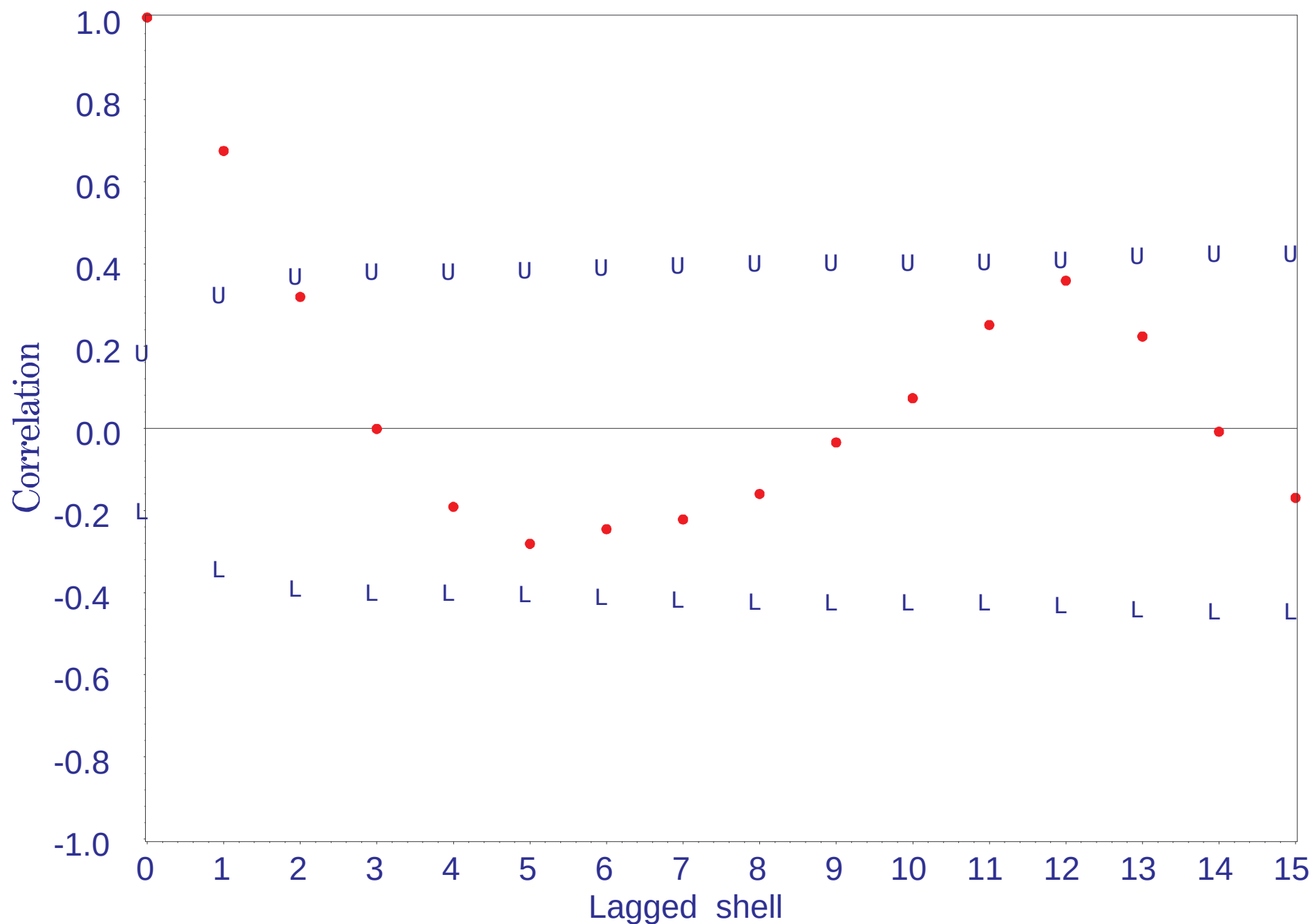
Shell Creek Flow (cfs) 1990-1998 Correlogram with Upper and Lower 95% Confidence Limits
