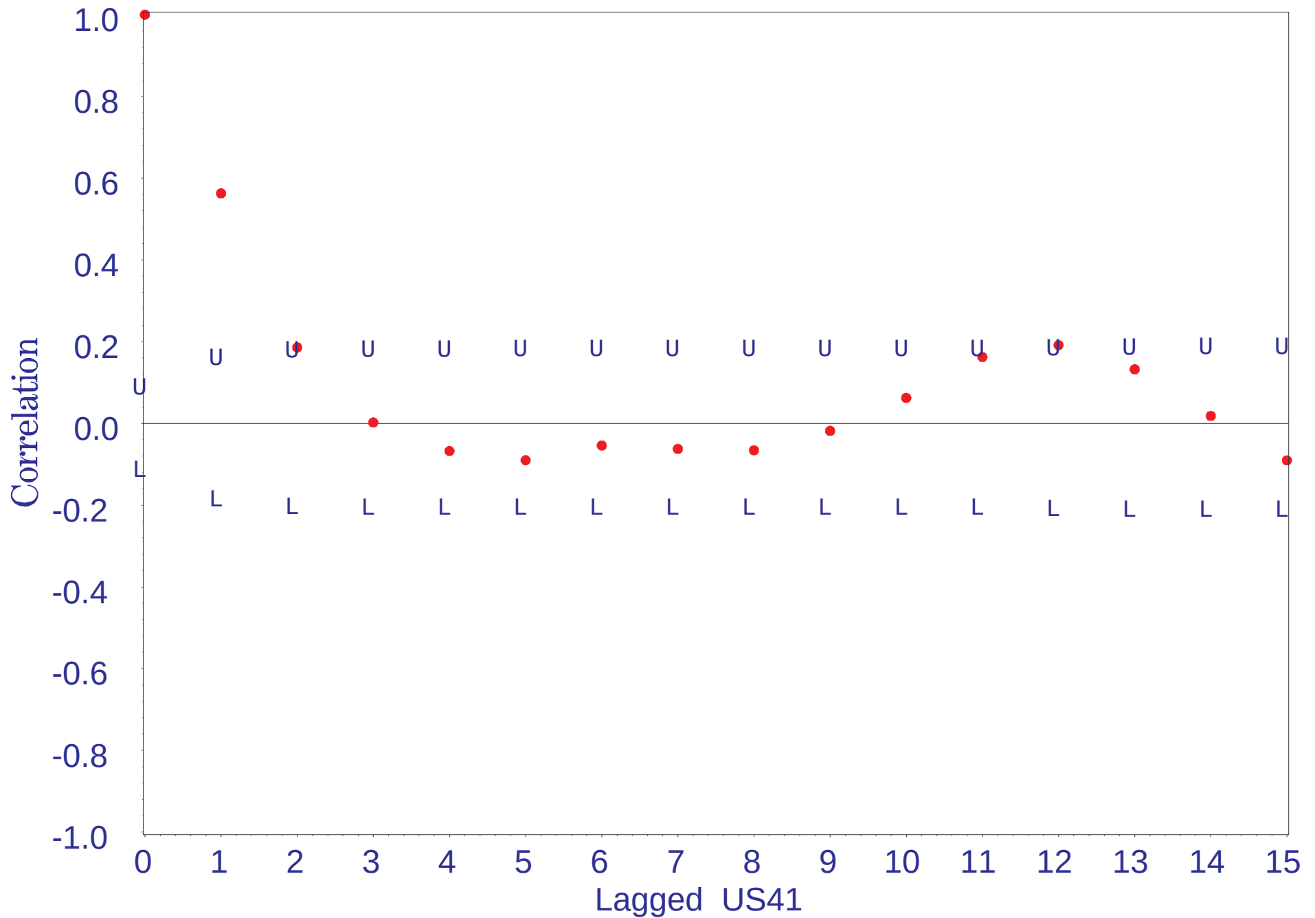
River Flow at US 41 Bridge 1966-1998 Correlogram with Upper and Lower 95% Confidence Limits
