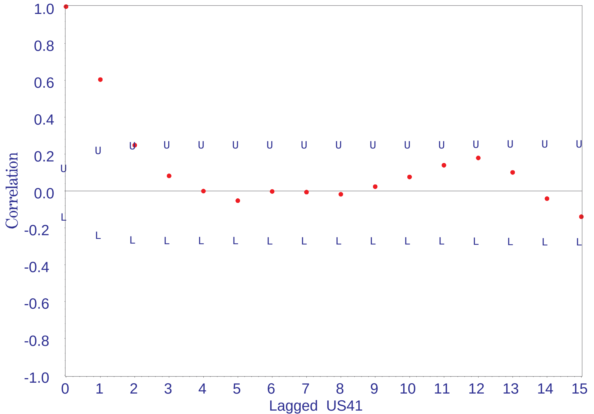
River Flow at US 41 Bridge 1980-1998 Correlogram with Upper and Lower 95% Confidence Limits
