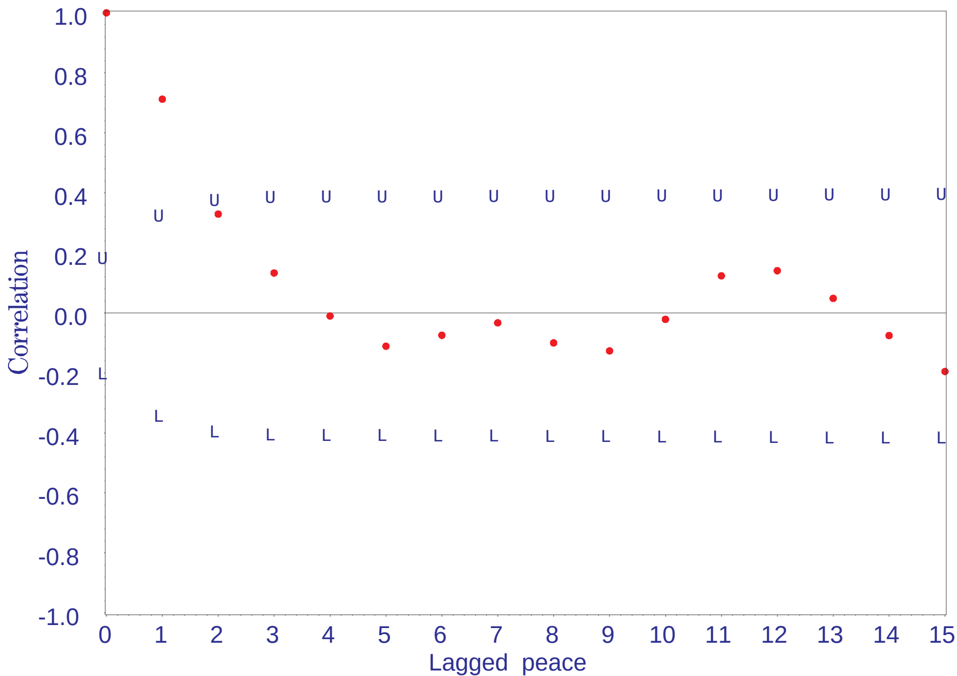
Peace River Flow at Archadia 1990-1998 Correlogram with Upper and Lower 95% Confidence Limits
