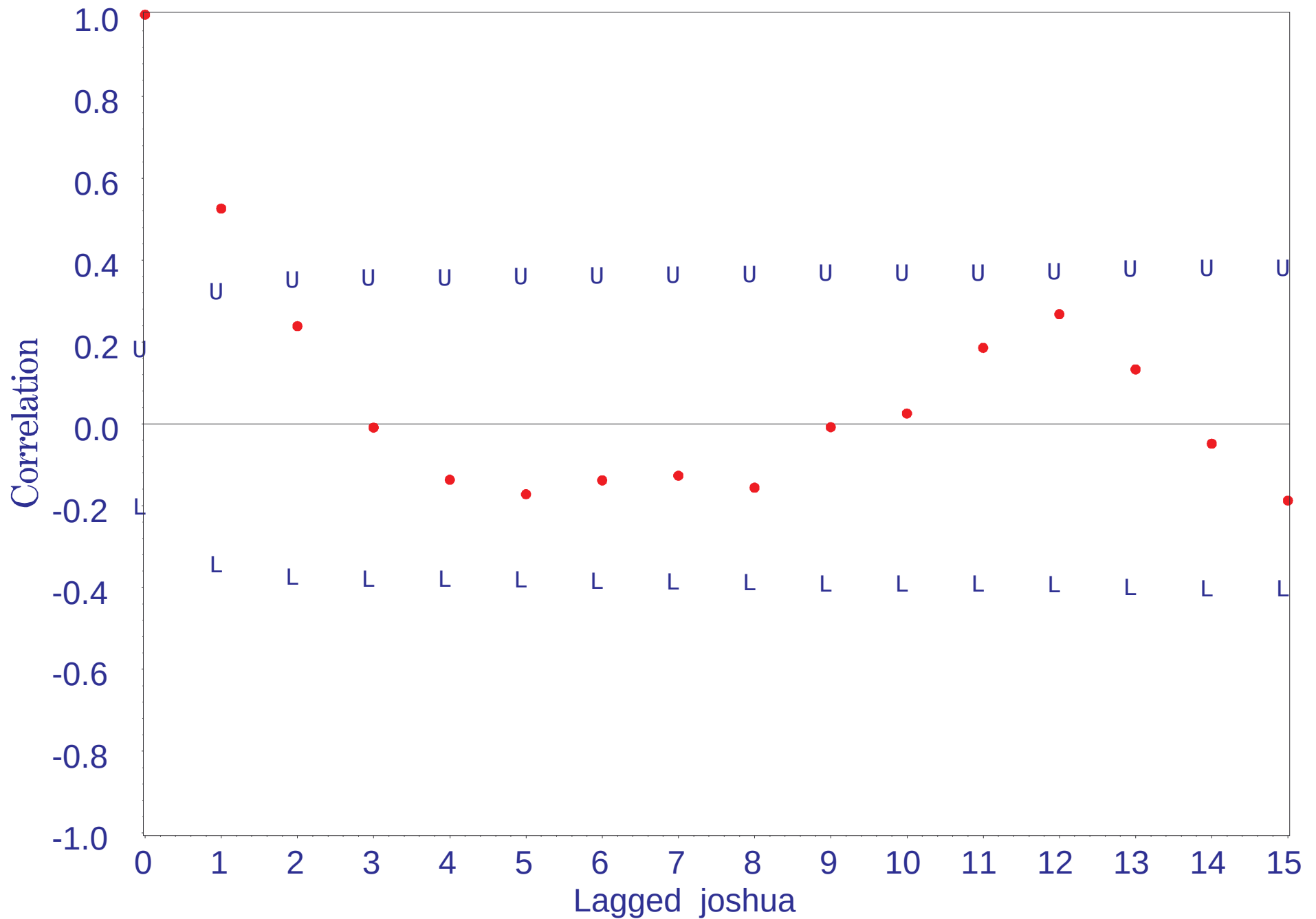
Joshua Creek Flow (cfs) 1990-1998 Correlogram with Upper and Lower 95% Confidence Limits
