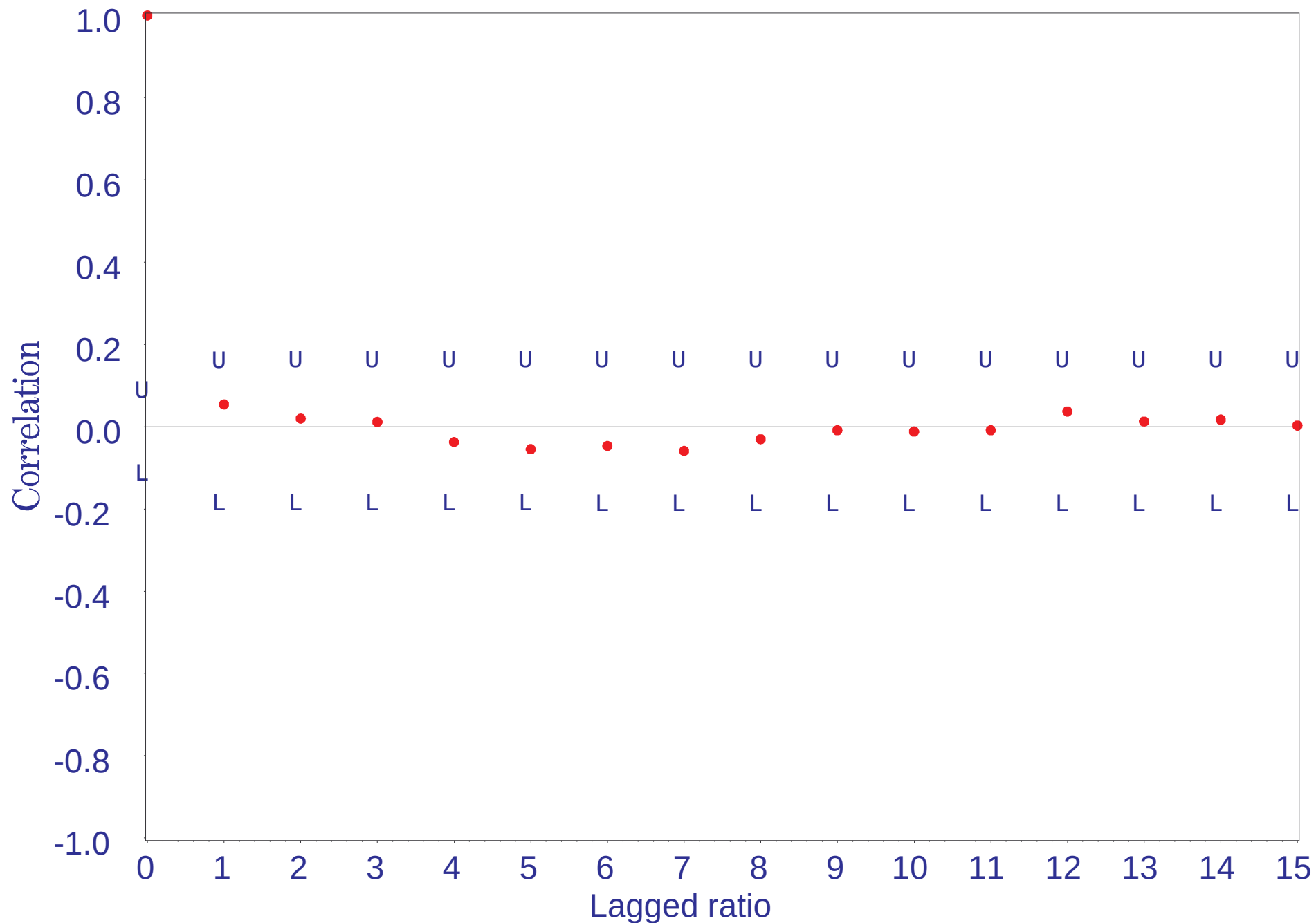
Ratio Arcadia Flow to Arcadia Rainfall (1966-1998) Correlogram with Upper and Lower 95% Confidence Limits
