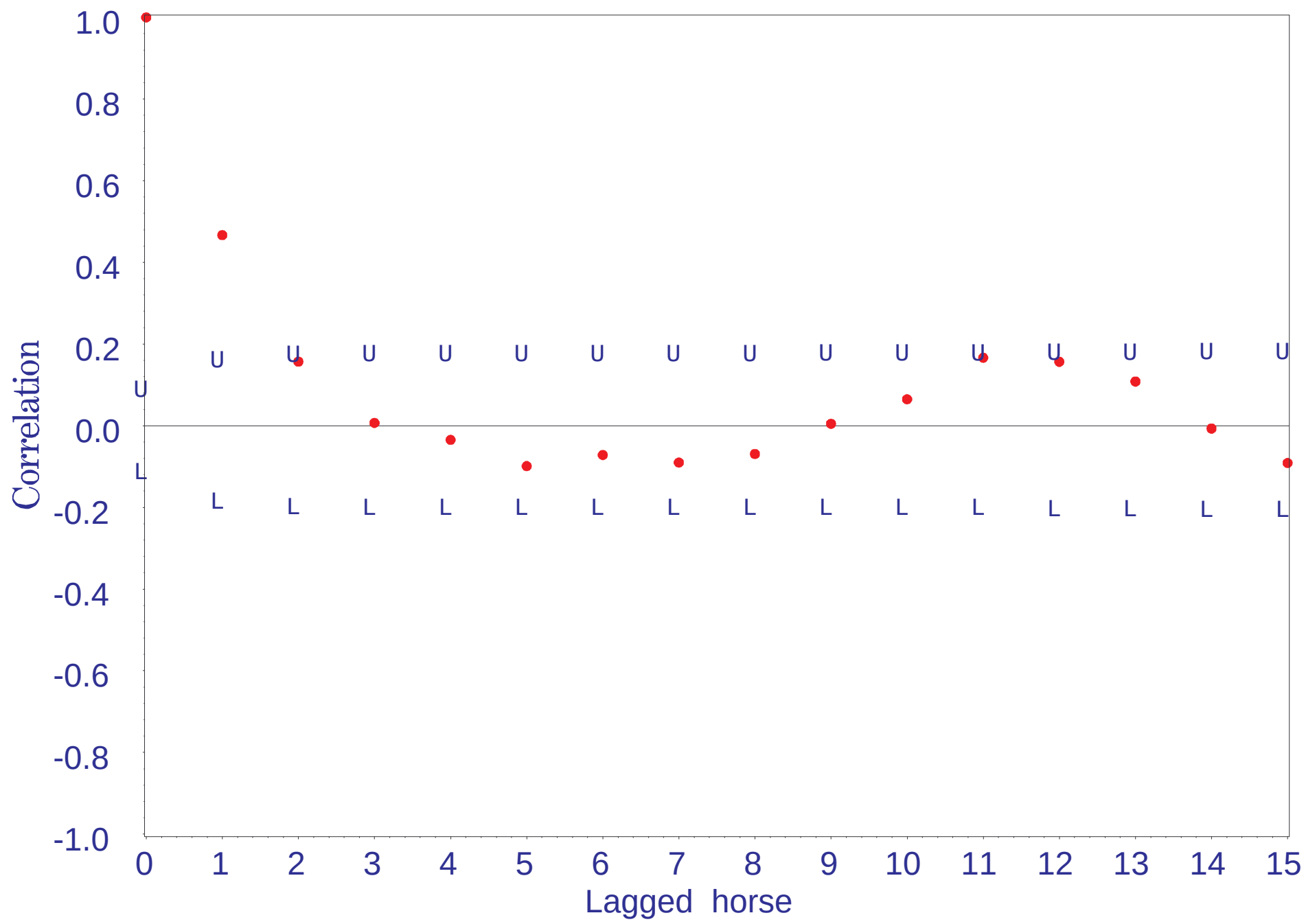
Horse Creek Flow (cfs) 1966-1998 Correlogram with Upper and Lower 95% Confidence Limits
