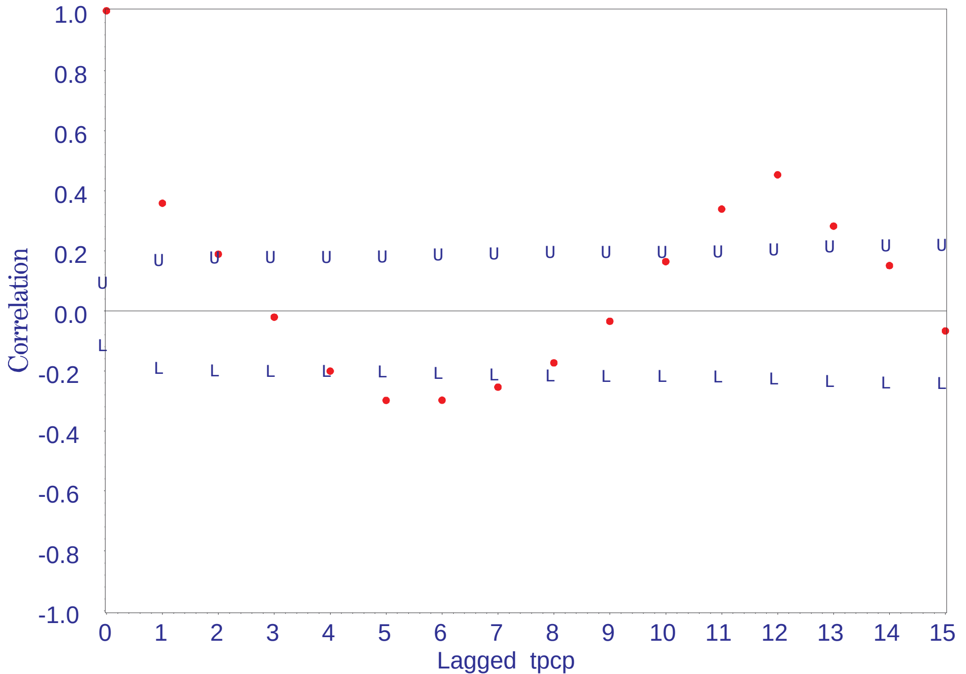
Monthly Rainfall at the Arcadia Gauge 1966-1998 Correlogram with Upper and Lower 95% Confidence Limits
