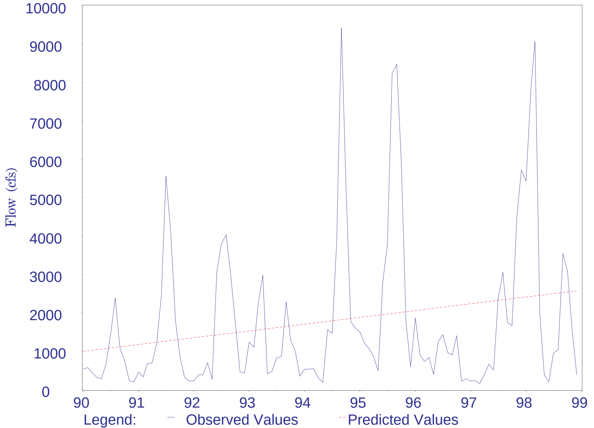
River Flow (cfs)at US 41 Bridge (1990-1998)
