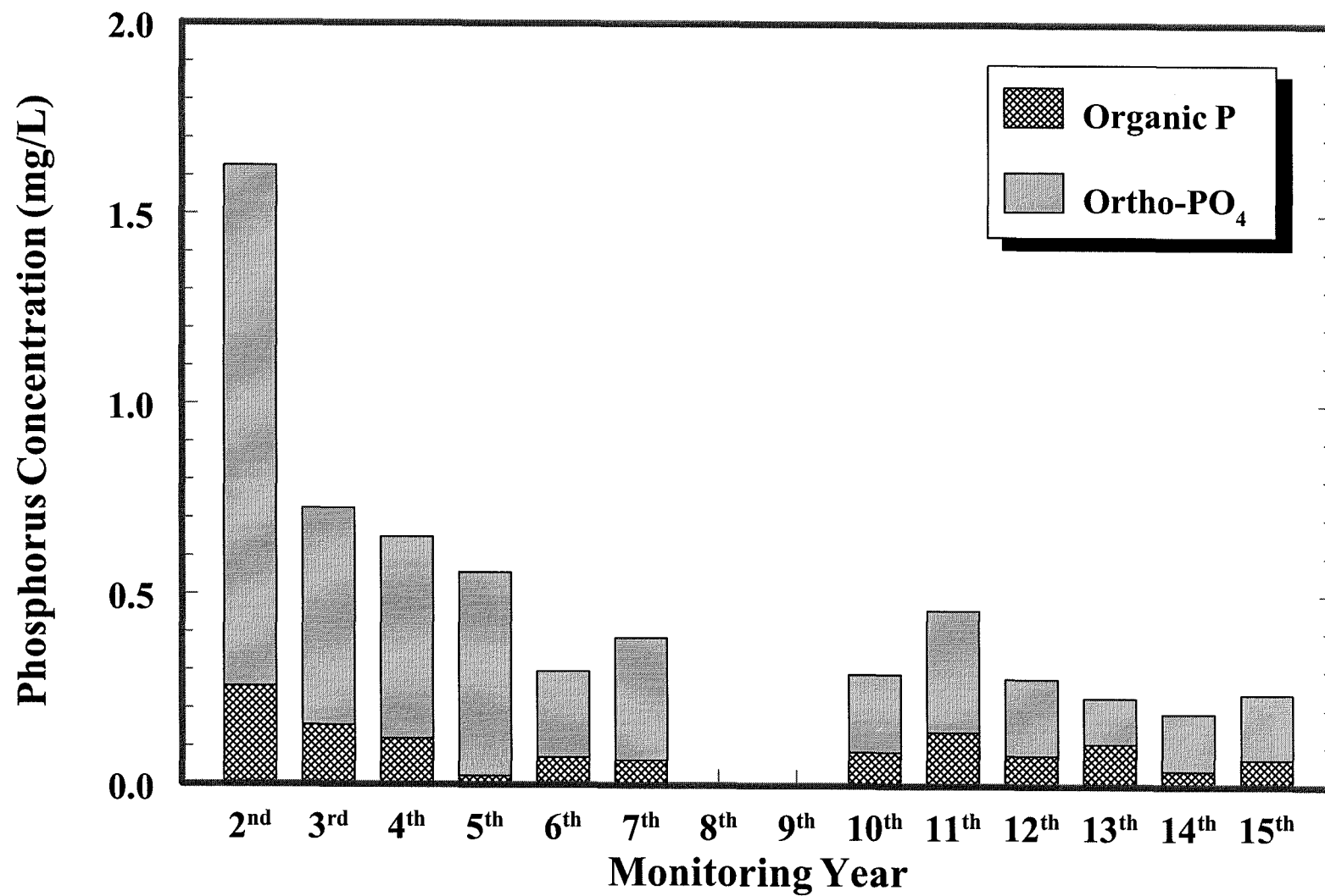
Figure 4.7. Average Phosphorus Concentrations Measured on the East Side of the Palmer Ranch from the Second through Fifteenth Monitoring Years
