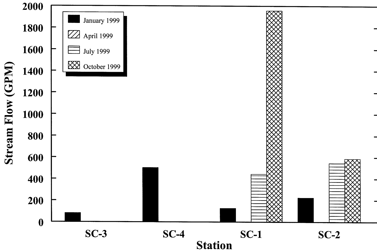
Figure 4.3. Stream Flows Measured during Monitoring Events Conducted on the East Side of the Palmer Ranch from January through December 1999
