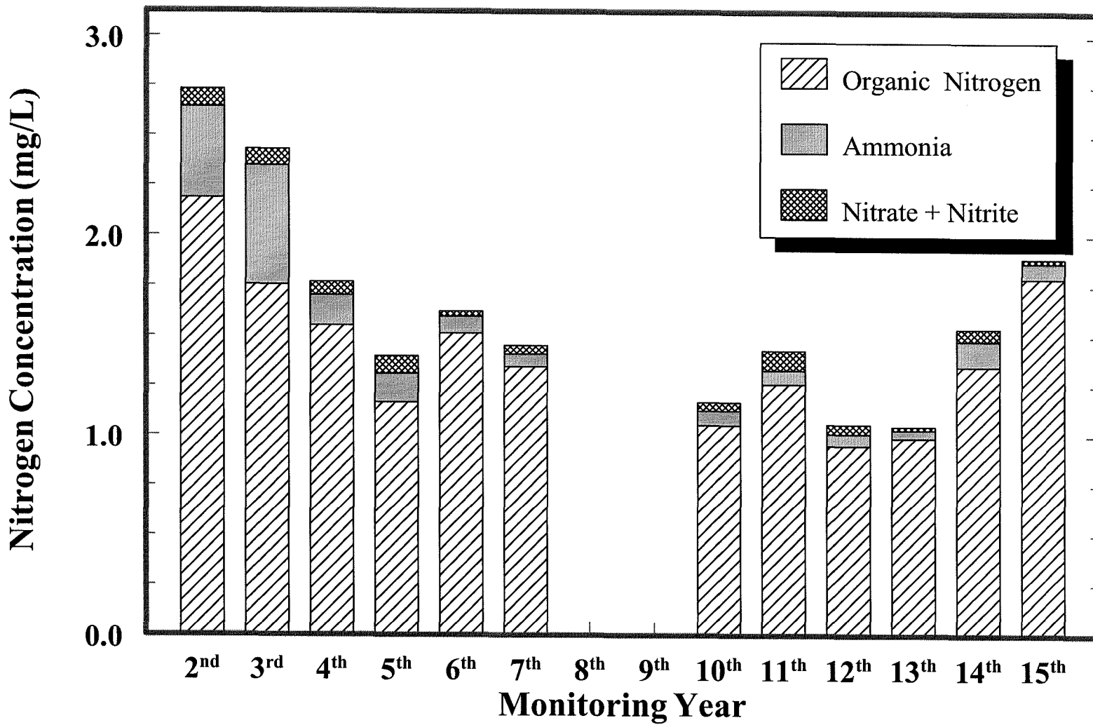
Figure 4.5. Average Nitrogen Concentrations Measured on the East Side of the Palmer Ranch from the Second through Fifteenth Monitoring Years
