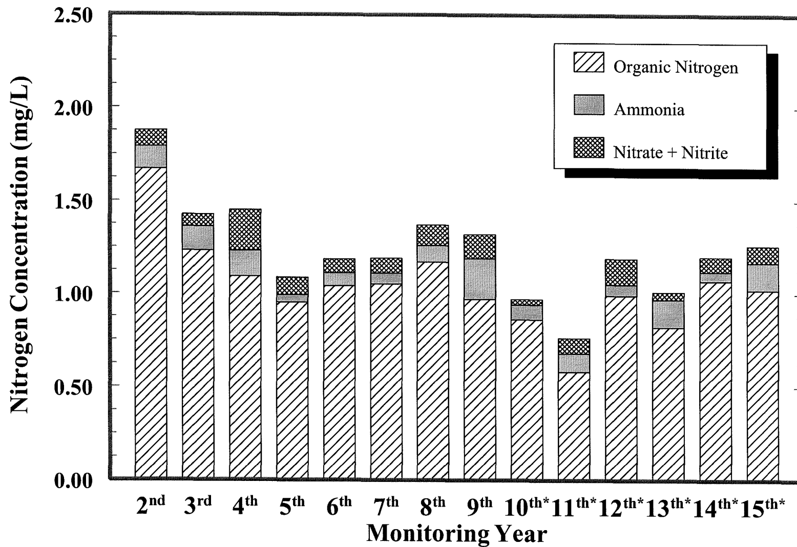
Figure 4.4. Average Nitrogen Concentrations Measured on the West Side of the Palmer Ranch from the Second through Fifteenth Monitoring Years
