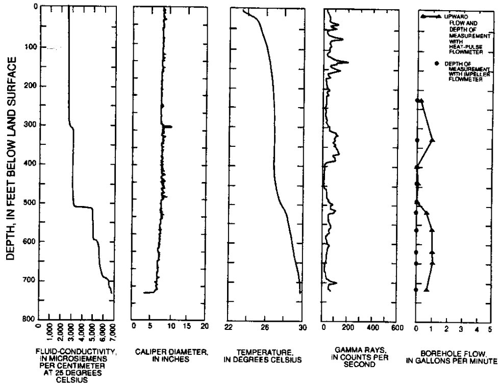
Figure 12. Composite geophysical log for Oscar Sherer State Park well in Sarasota County.
