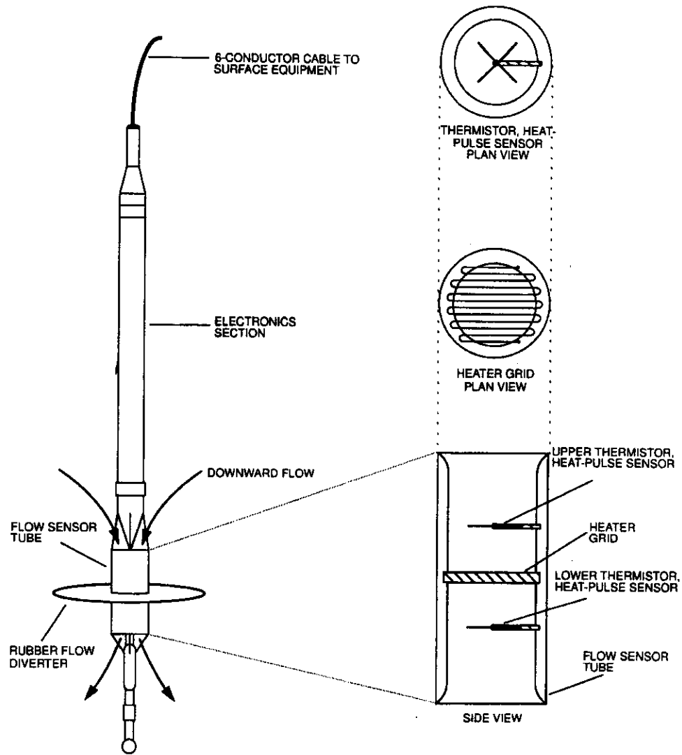
Figure 8. The components of the heat-pulse flowmeter (modified from Hess, 1990).
