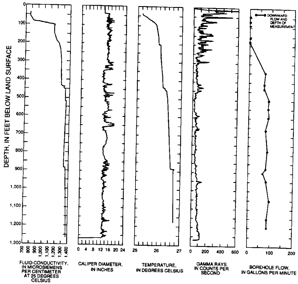
Figure 13. Composite geophysical log for Utopia No. 1 well in Sarasota County.
