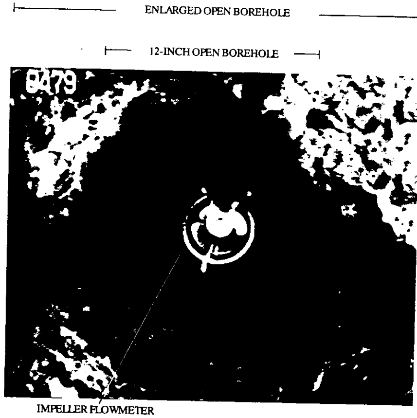
Figure 7. A borehole video camera with the impeller flowmeter attachment in a 12-inch open borehole at a depth of 479 feet below land surface.
