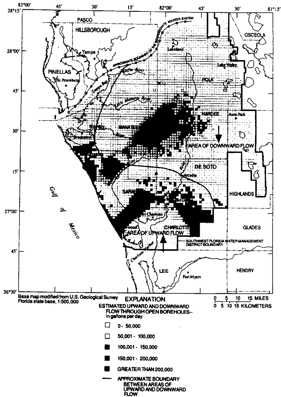
Figure 27. Grid network with cumulative downward and upward flow rates for wells open to both the intermediate aquifer system and the Upper Floridan aquifer.
