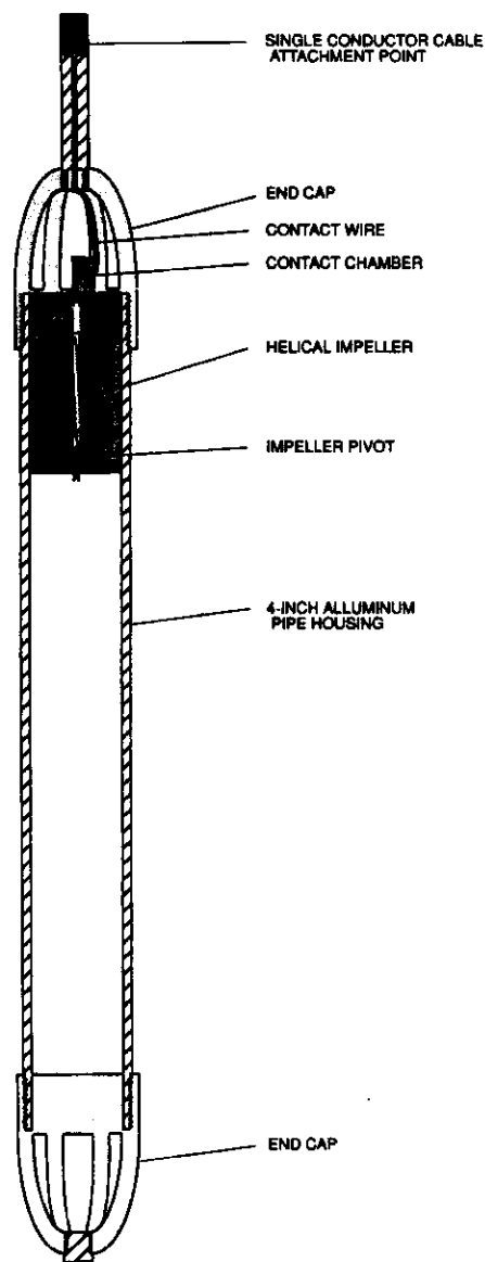
Figure 6. The components of the impeller flowmeter.
