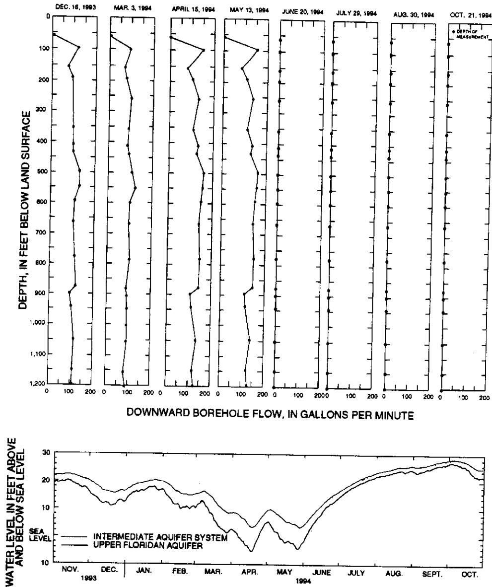
Figure 16. Seasonal flow measurements for Utopia No. 1 well in Sarasota County and hydrographs of the intermediate aquifer system and the Upper Floridan aquifer, November 1993 through October 1994.
