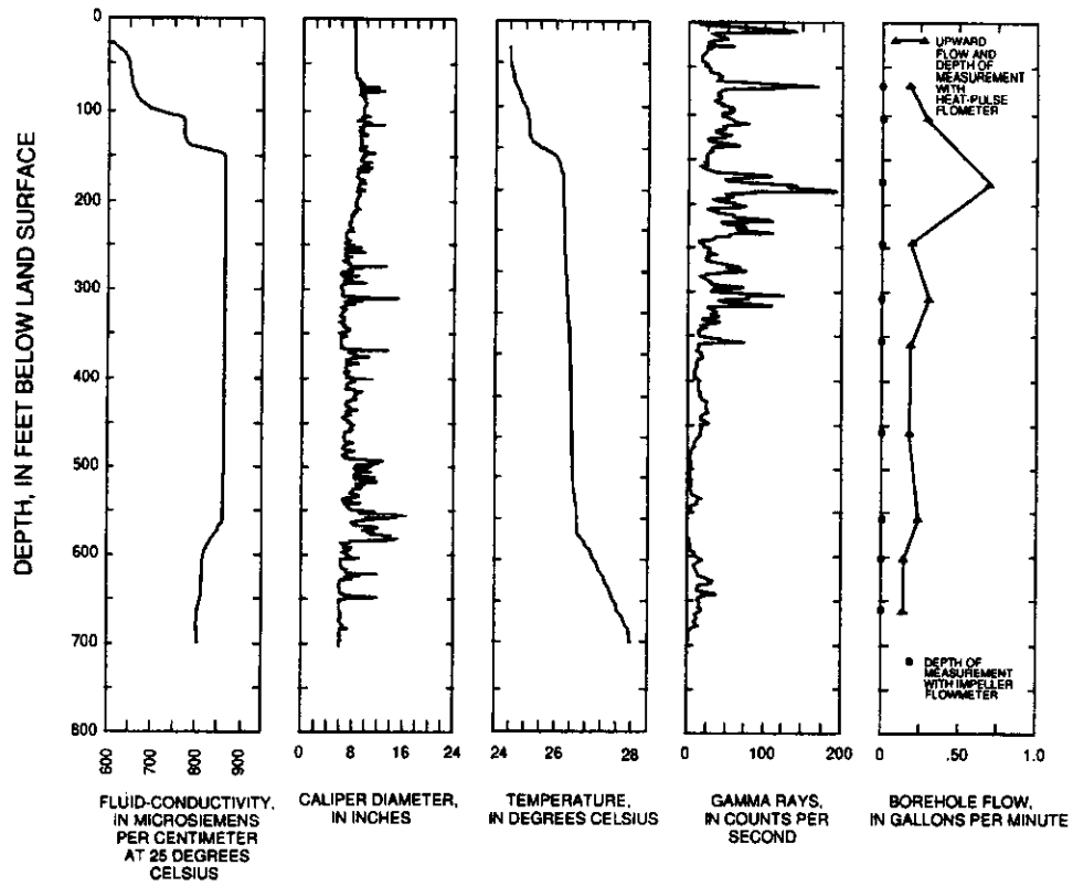
Figure 18. Composite geophysical log for Schroeder Manatee Ranch No. 8 well in Manatee County using the heat-pulse flowmeter.
