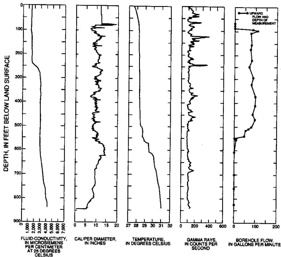
Figure 11. Composite geophysical log for ROMP 20 well in Sarasota County.
