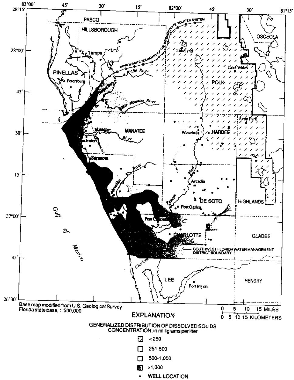
Figure 23. Generalized distribution of dissolved solids in water from the intermediate aquifer system.
