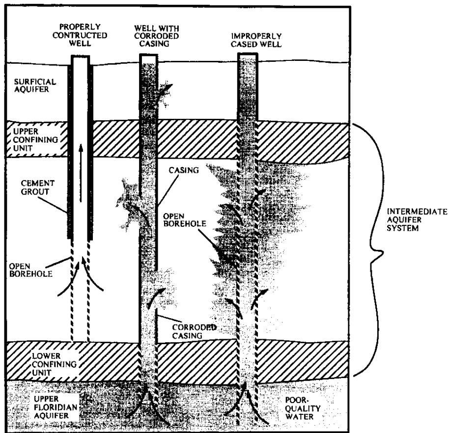
Figure 3. A properly constructed well open to a single aquifer, and a corroded well and an improperly constructed well that can allow water quality contamination between multiple aquifers.
