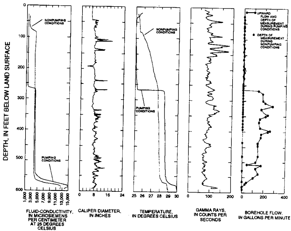
Figure 16. Composite geophysical log for Hickory Street well in Sarasota County with Production No. 3 well under nonpumping and pumping conditions.
