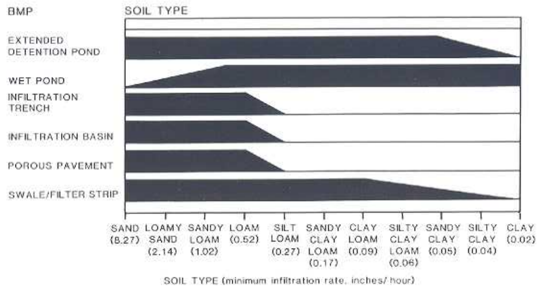
Figure 7: BMPs FOR DIFFERENT SOIL TYPES
