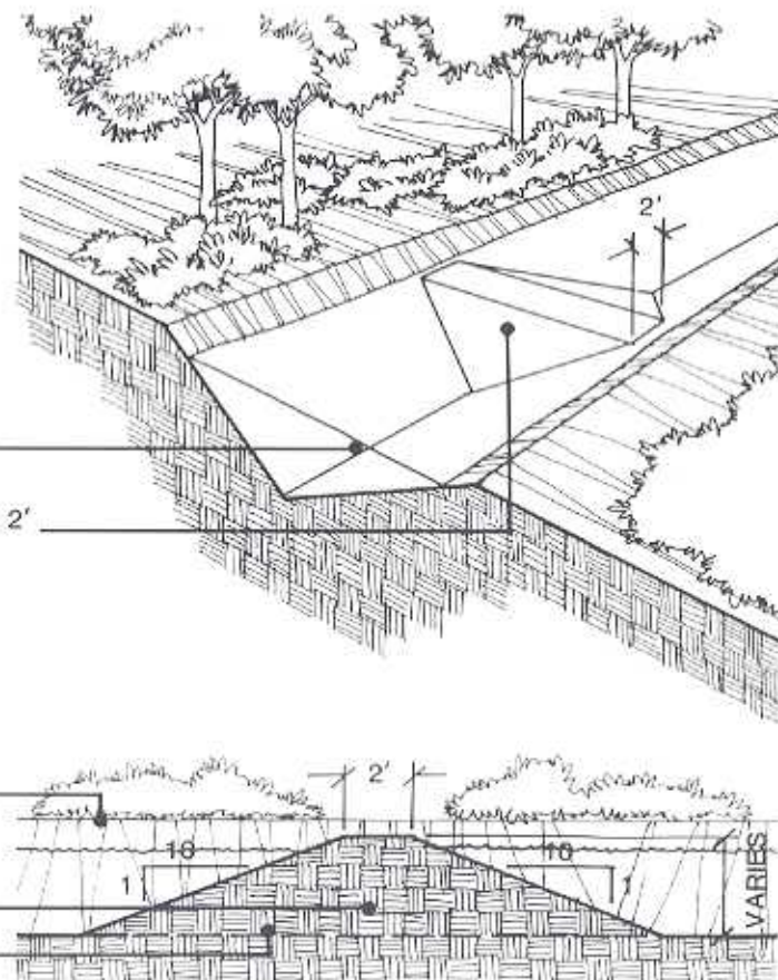
Figure 11: SWALE WITH CROSS BLOCK
