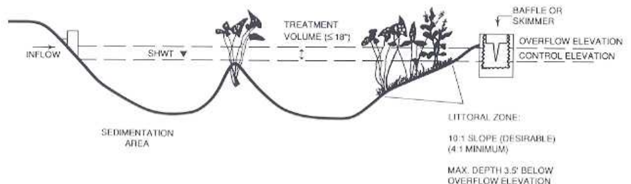
Figure 12: TYPICAL WET DETENTION COMPONENTS
